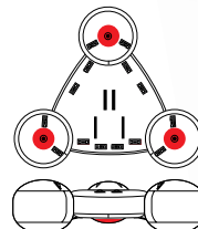
ATOM
